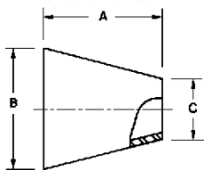
31W CONCENTRIC REDUCER
