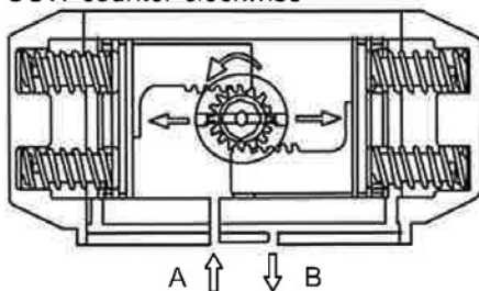
Air to port A forces the pistons outwards, causing the springs to compress. The pinion turns counter-clockwise while air is being exhausted through port B.
