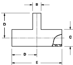
7WR REDUCING TEE
