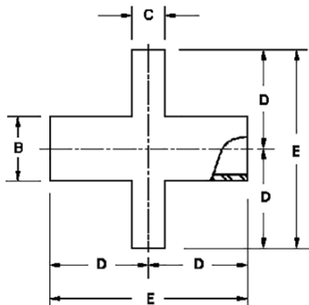
9WR REDUCING CROSS
