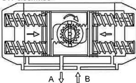
Loss of air pressure through port A allows the springs to force the pistons inwards. The pinion turns clockwise while air is being exhausted through port A.
