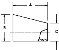
32W ECCENTRIC REDUCER
