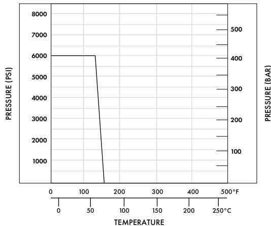
PRESSURE/TEMP. RATING
