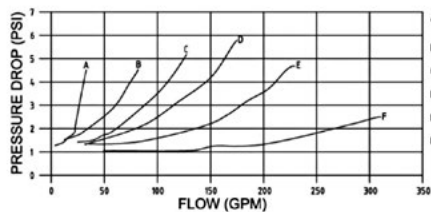
Spring Check Valve Pressure Drop
